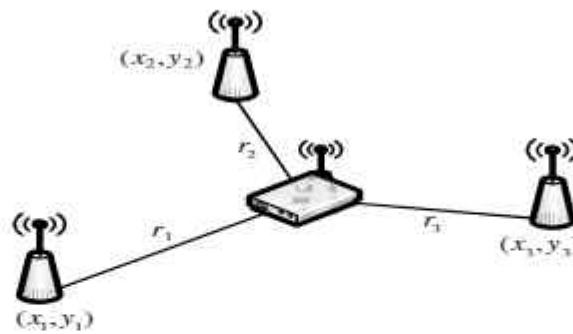
Fig.3. Lateration method using three anchor nodes
